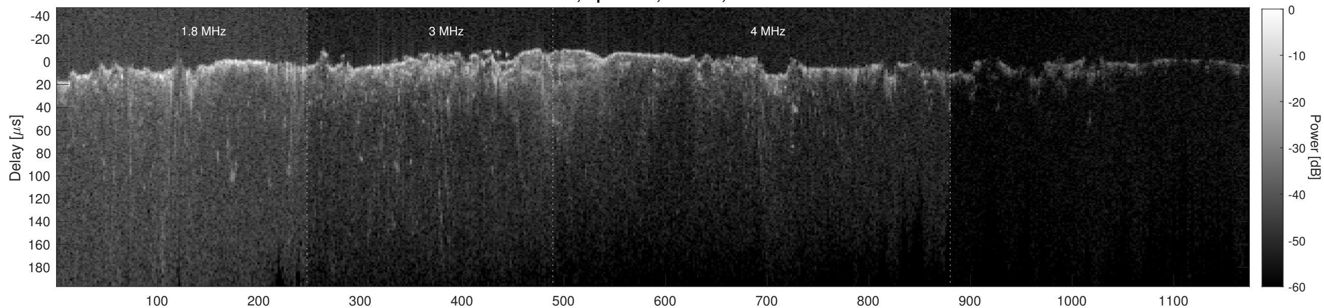
Orbit 2541, Cluttergram
