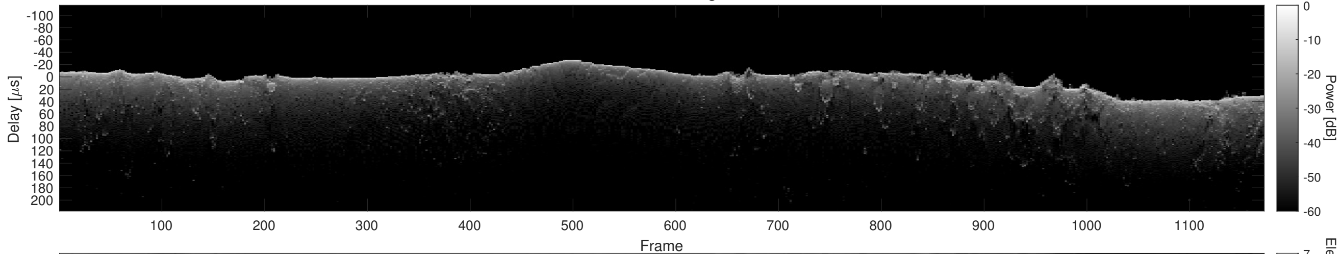
Orbit 2543, Cluttergram
