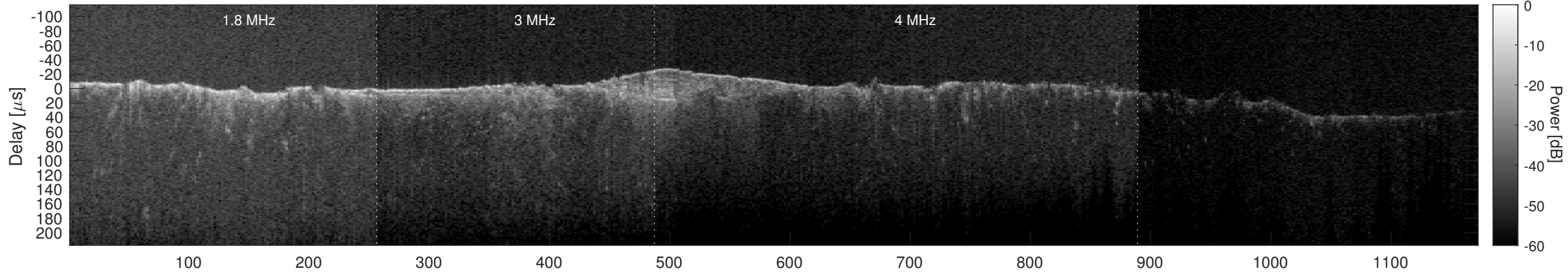
Orbit 2543, Cluttergram
