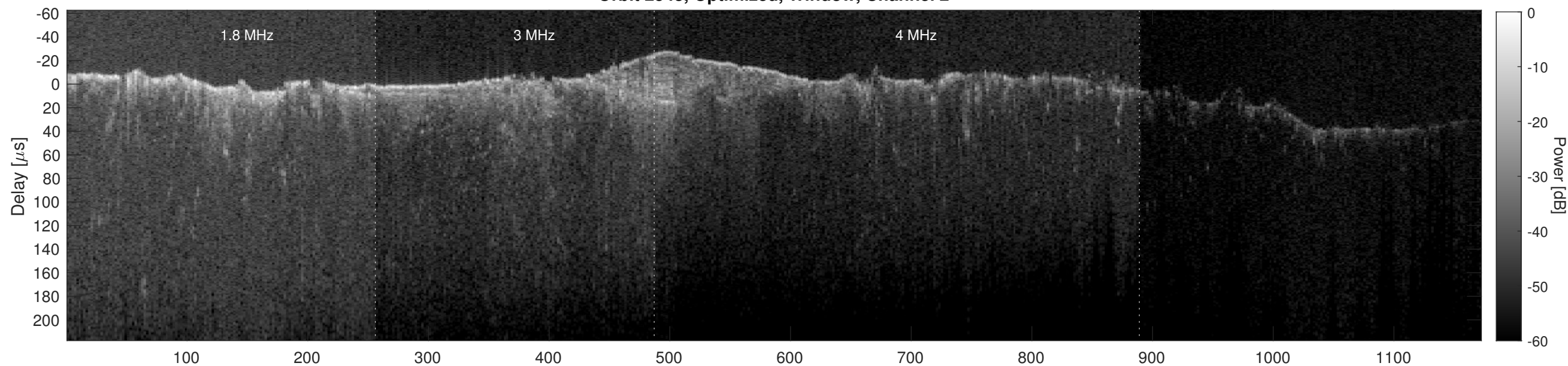
Orbit 2543, Cluttergram
