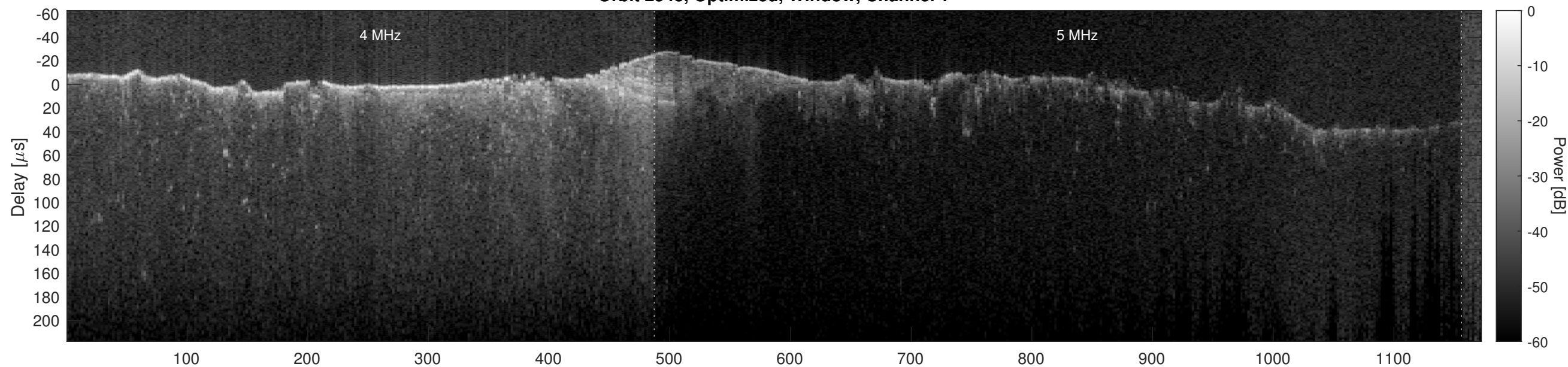
Orbit 2543, Optimized, Window, Channel 2
