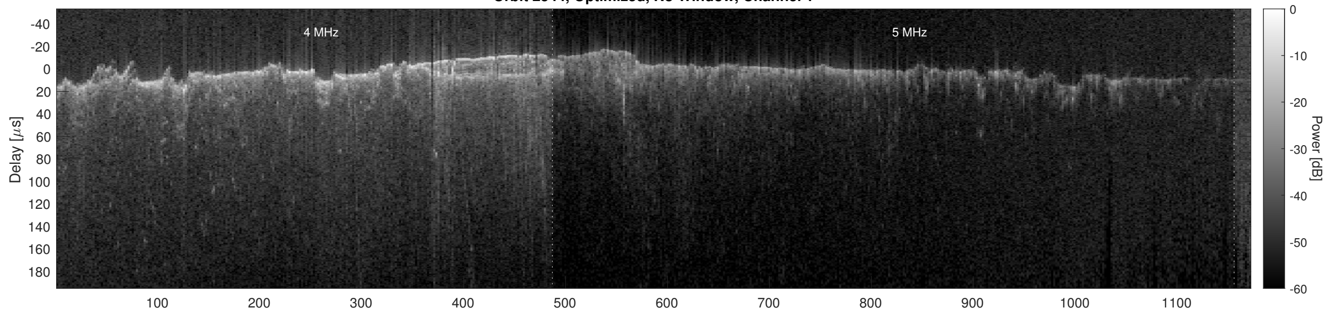
Orbit 2544, Optimized, No Window, Channel 2
