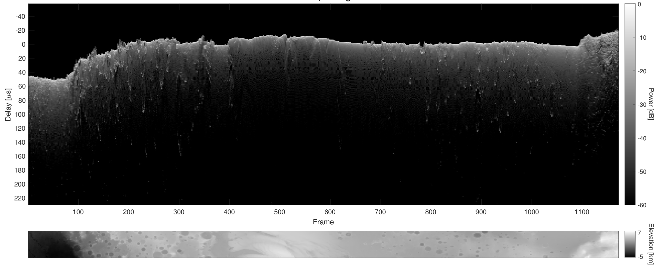
Orbit 2545, Cluttergram
