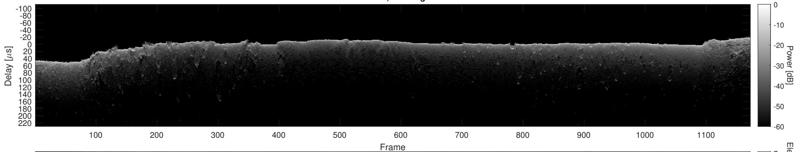
Orbit 2545, Cluttergram
