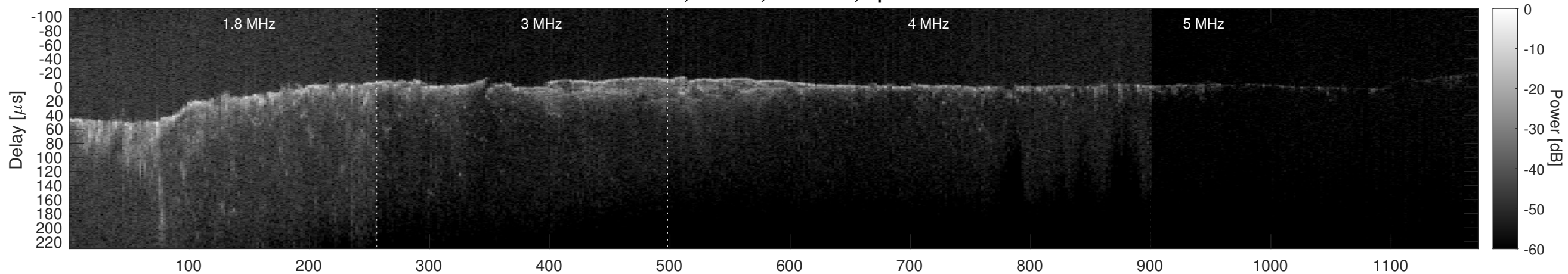
Orbit 2545, Cluttergram
