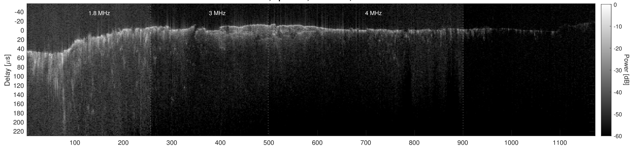
Orbit 2545, Cluttergram
