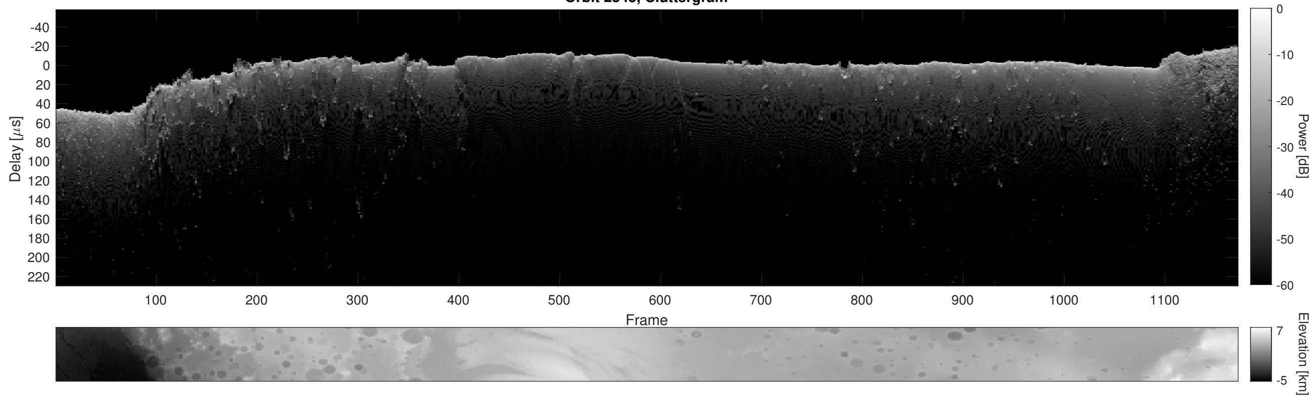
Orbit 2545, Cluttergram
