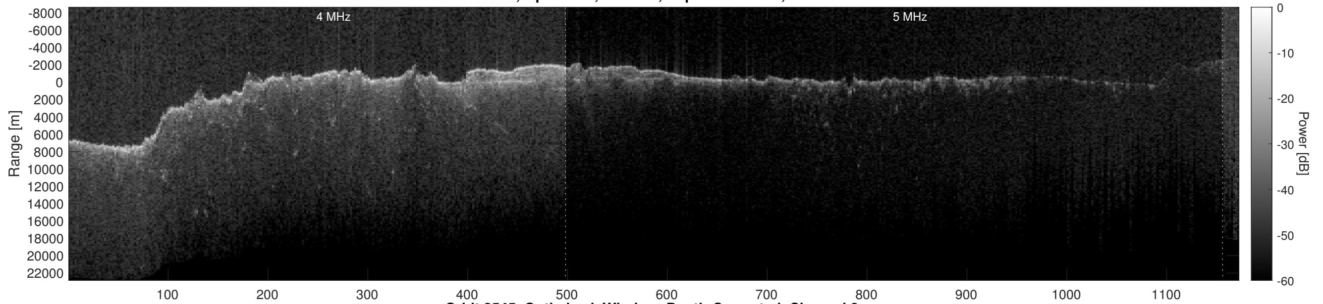
Orbit 2545, Optimized, Window, Depth-Corrected, Channel 2
