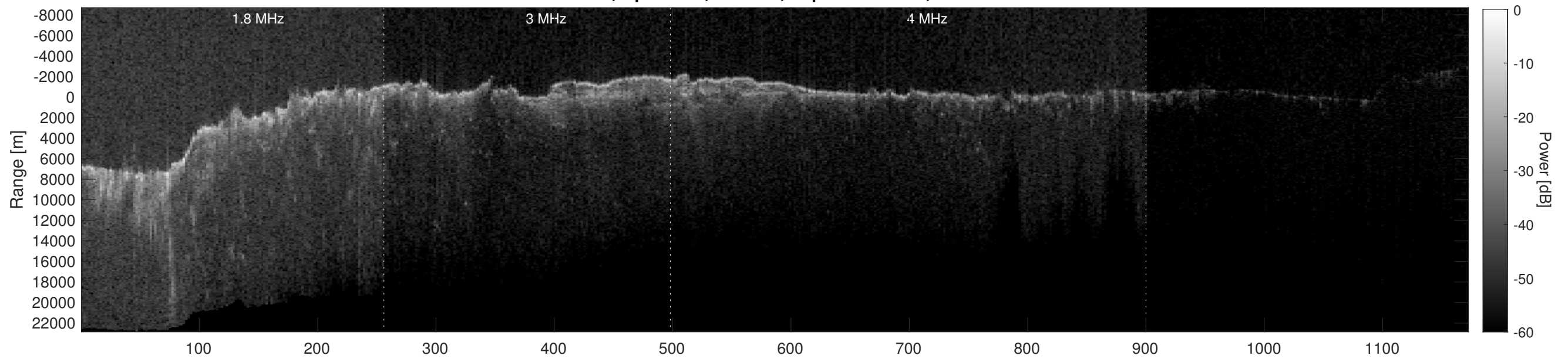
Orbit 2545, Depth-Corrected Cluttergram
