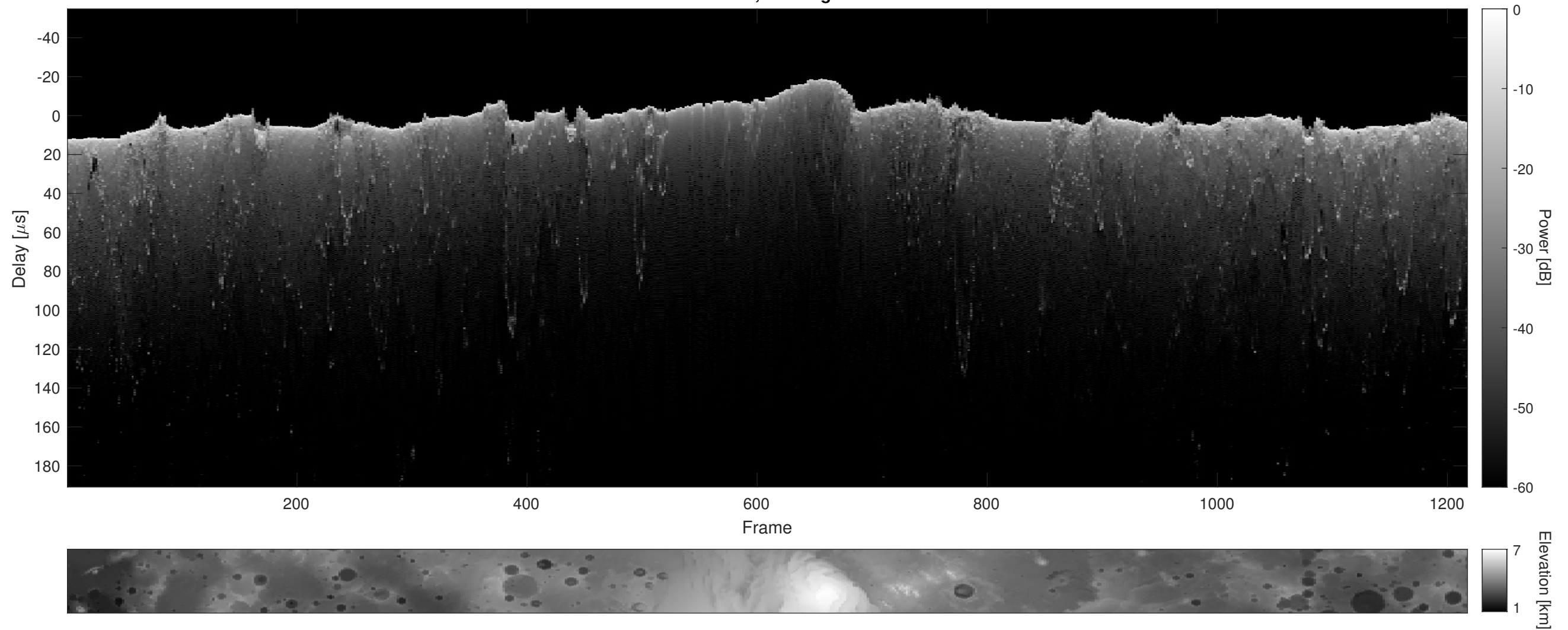
Orbit 2573, Cluttergram
