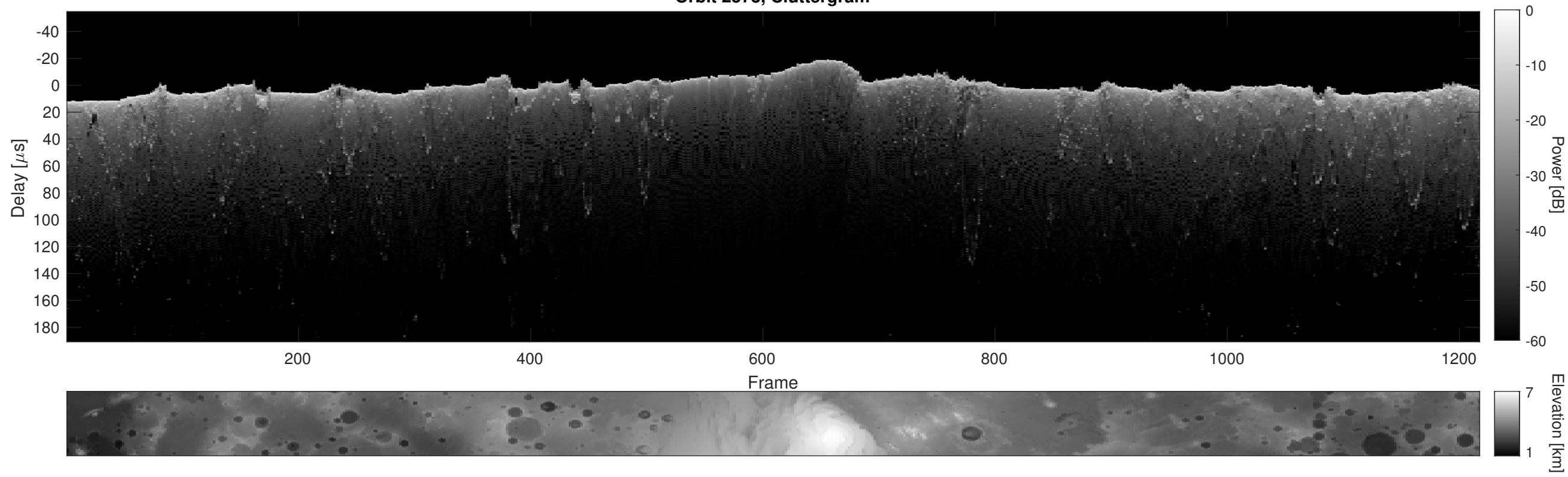
Orbit 2573, Cluttergram
