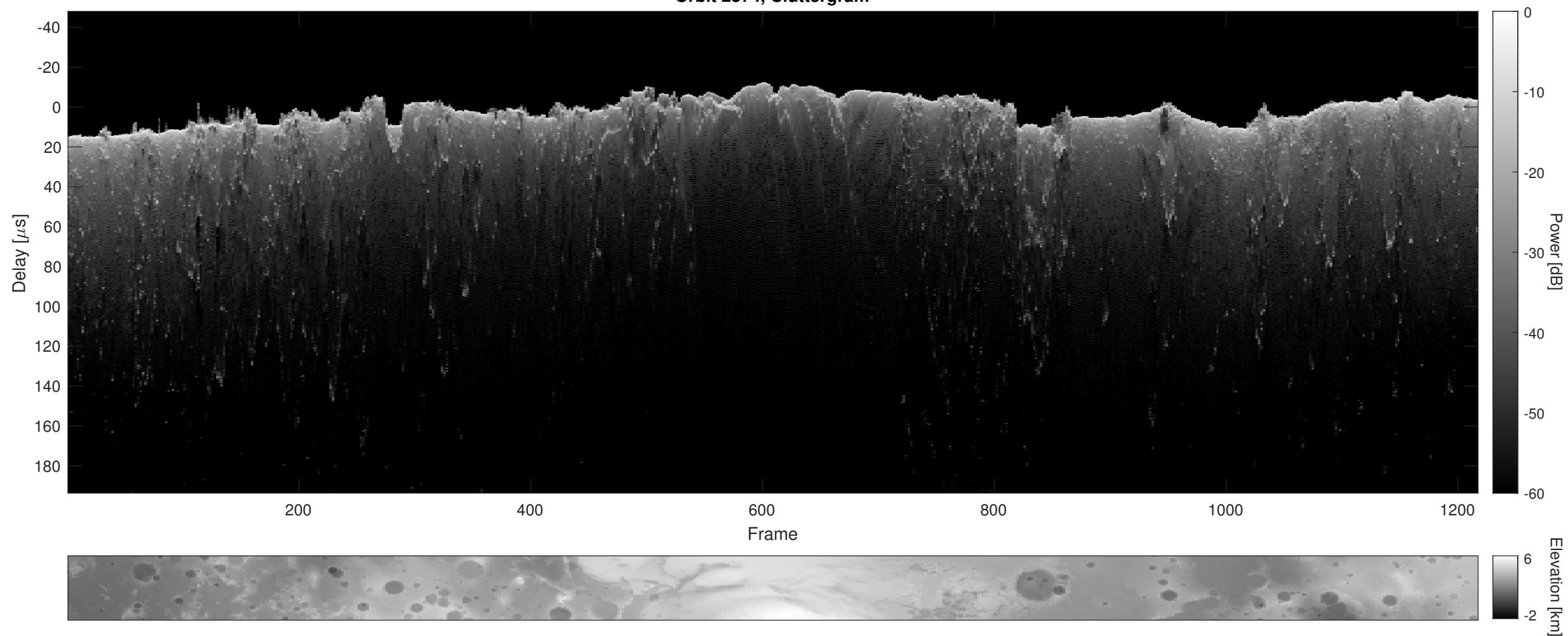
Orbit 2574, Cluttergram
