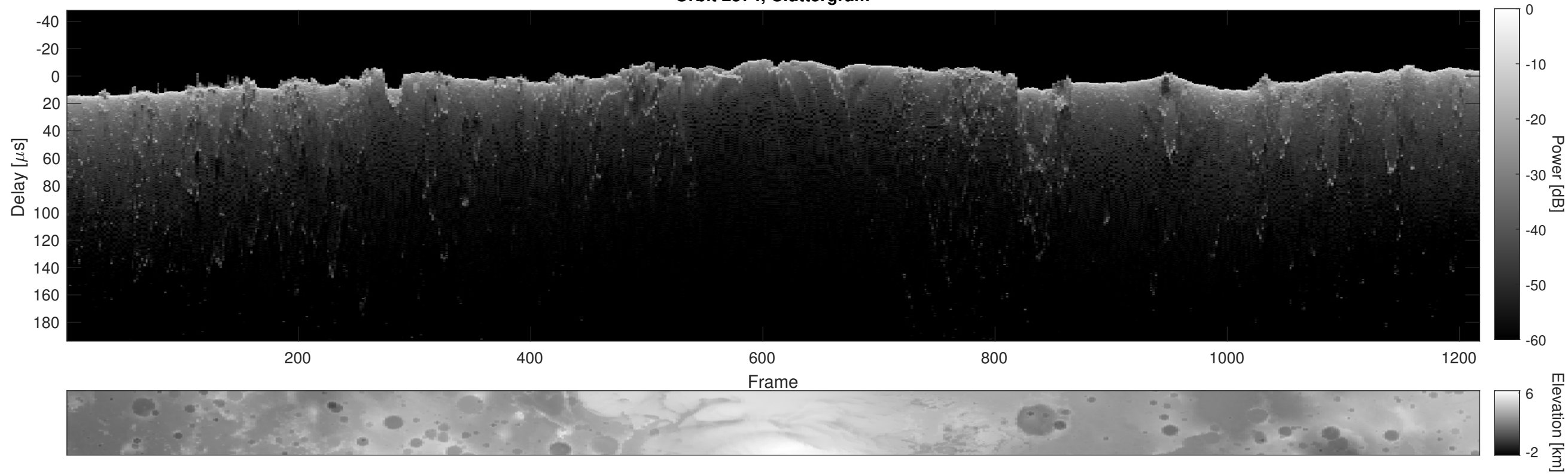
Orbit 2574, Cluttergram
