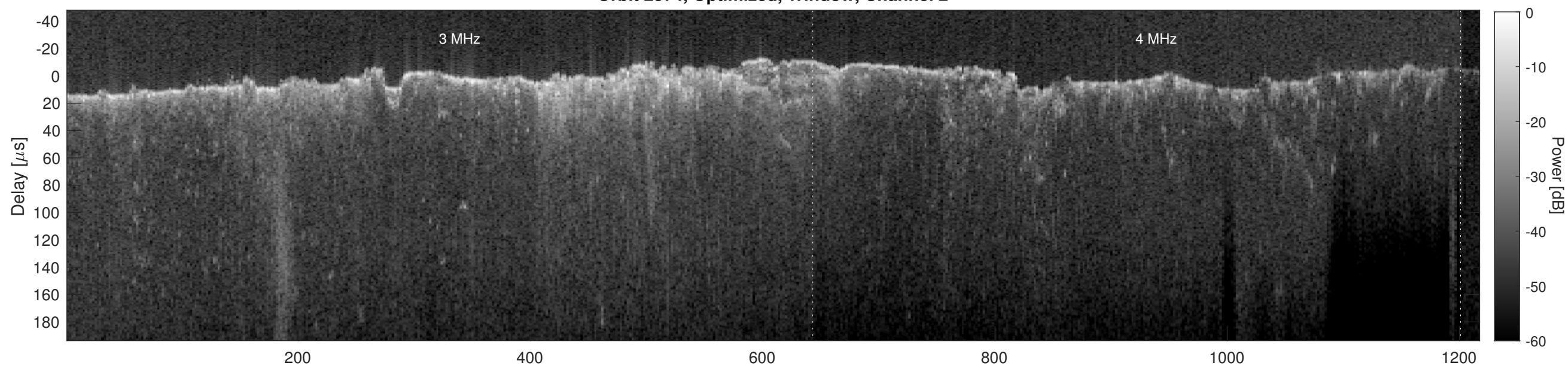
Orbit 2574, Cluttergram
