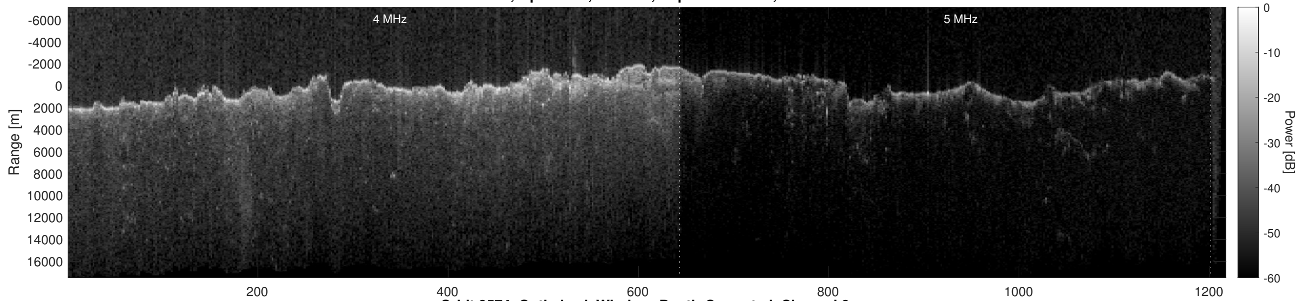
Orbit 2574, Optimized, Window, Depth-Corrected, Channel 2
