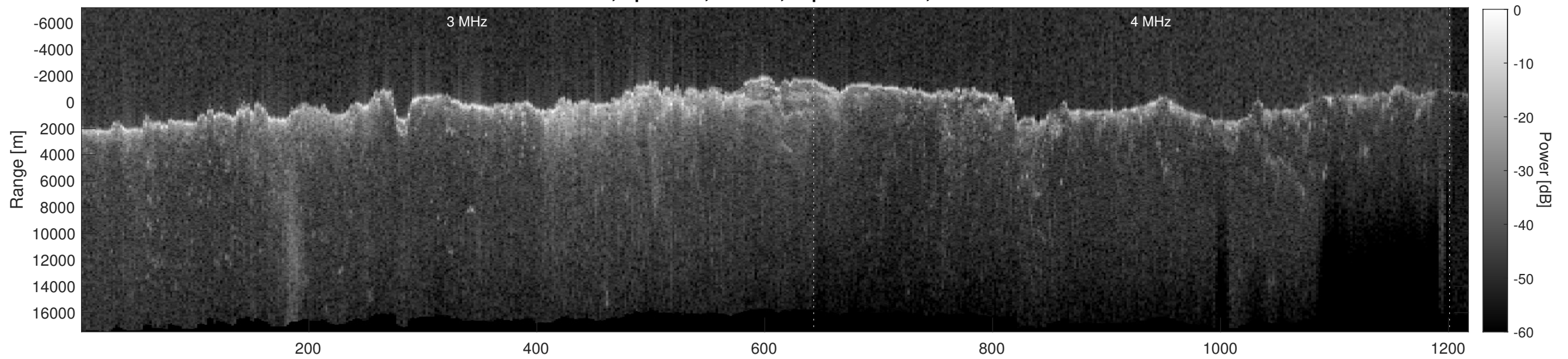
Orbit 2574, Depth-Corrected Cluttergram
