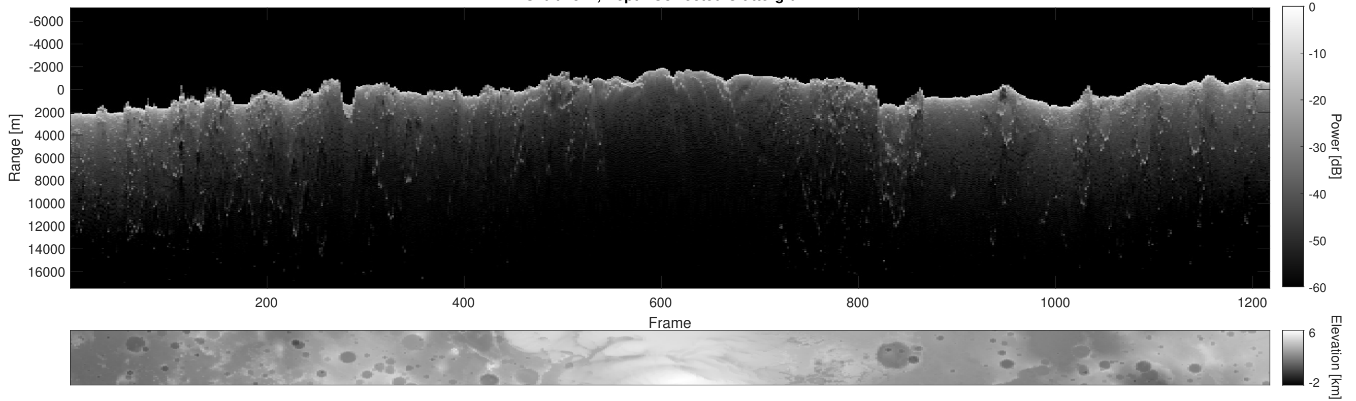
Orbit 2574, Depth-Corrected Cluttergram
