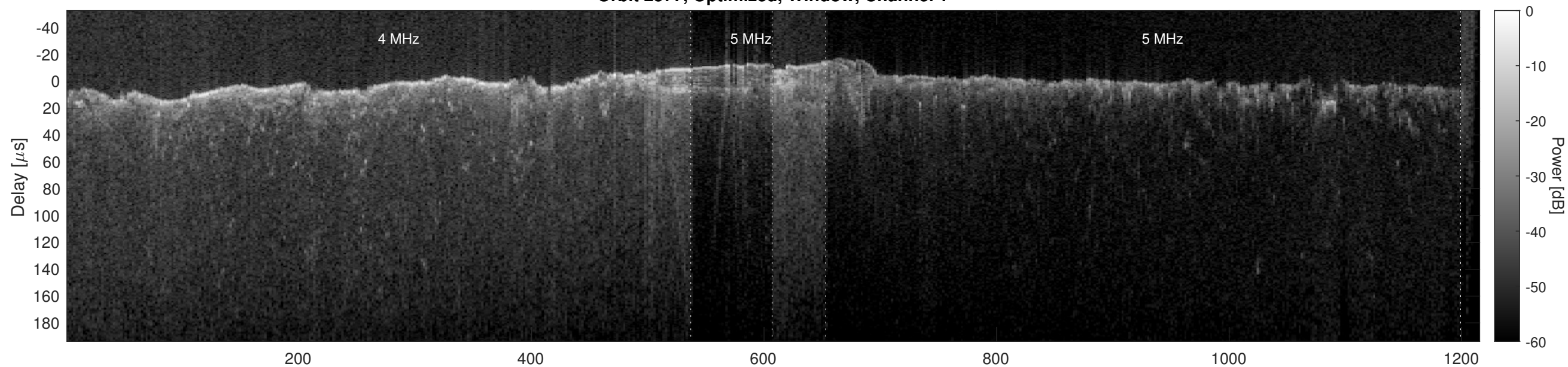
Orbit 2577, Optimized, Window, Channel 2
