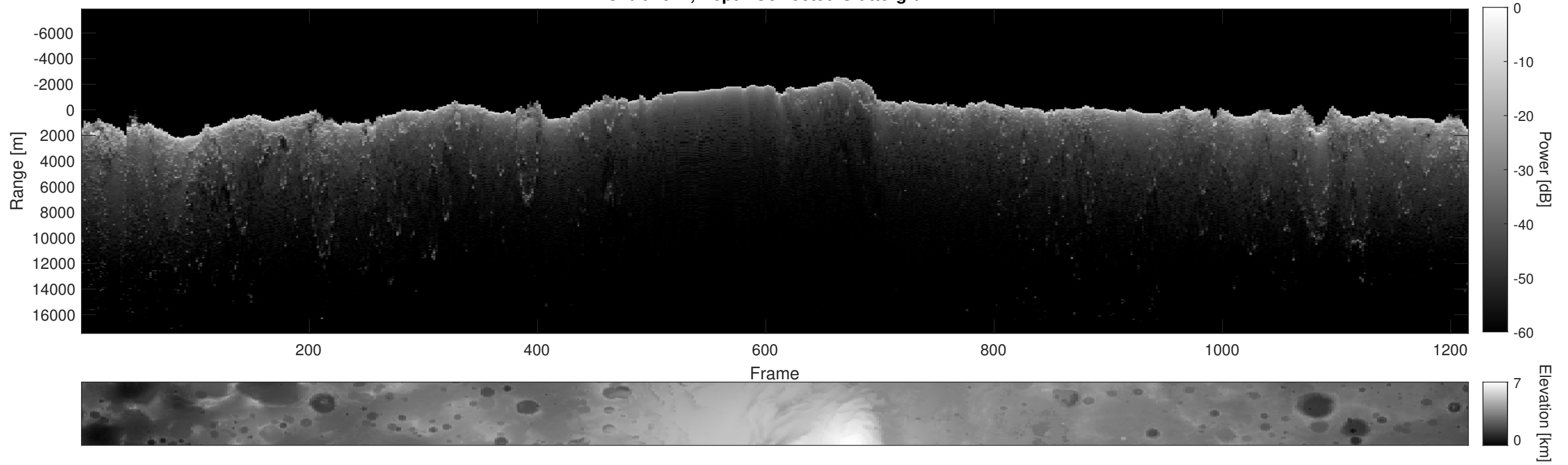
Orbit 2577, Depth-Corrected Cluttergram
