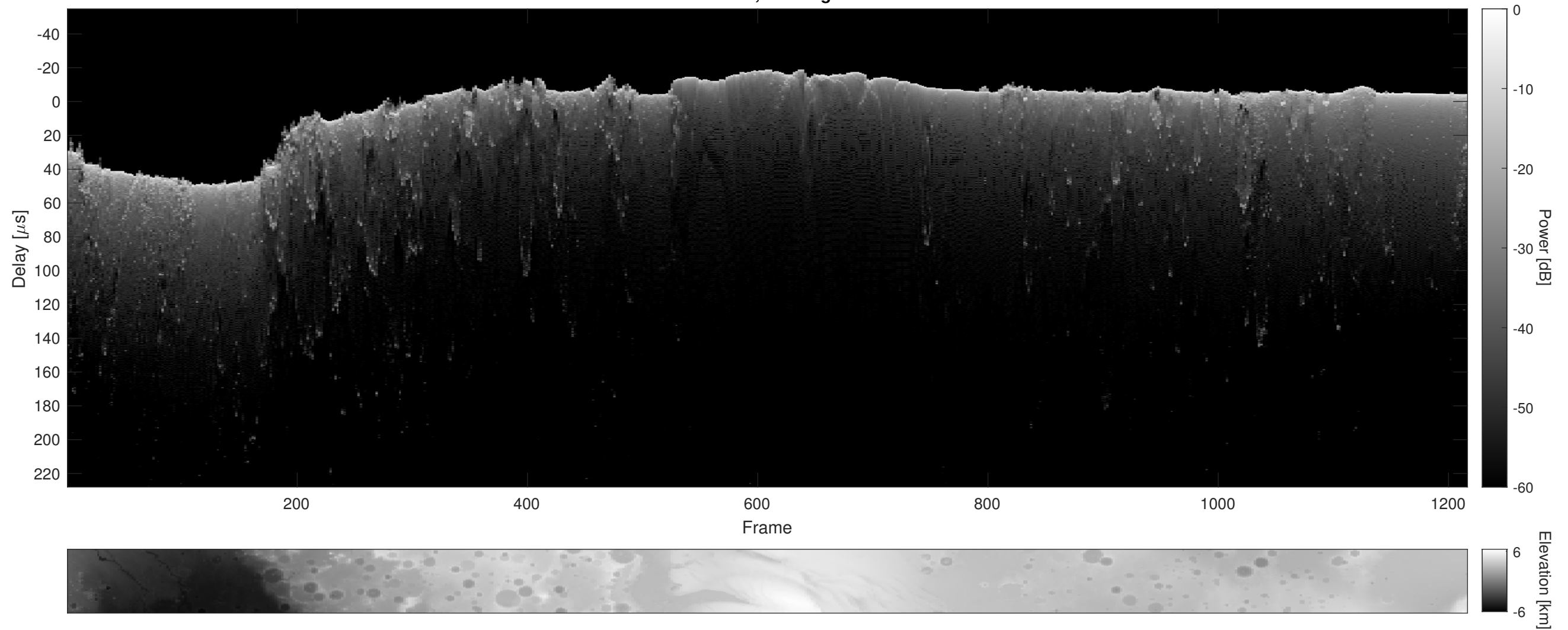
Orbit 2578, Cluttergram
