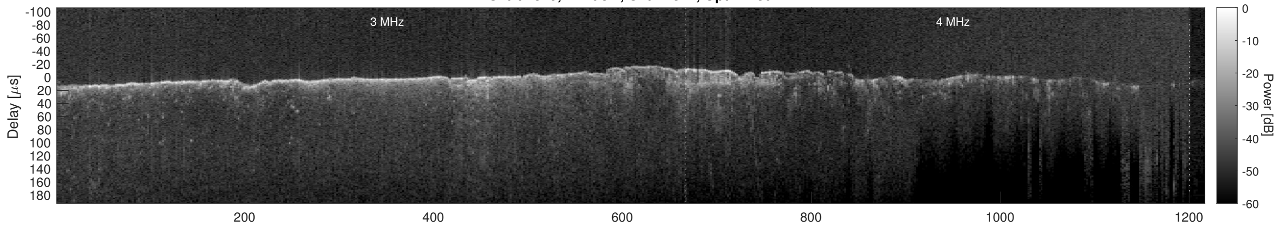
Orbit 2579, Cluttergram
