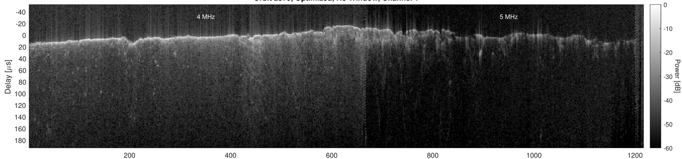
Orbit 2579, Optimized, No Window, Channel 2
