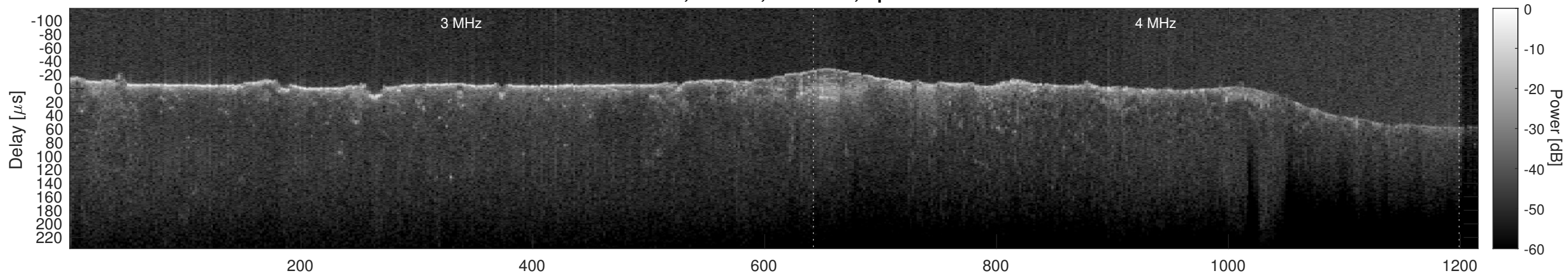
Orbit 2580, Cluttergram
