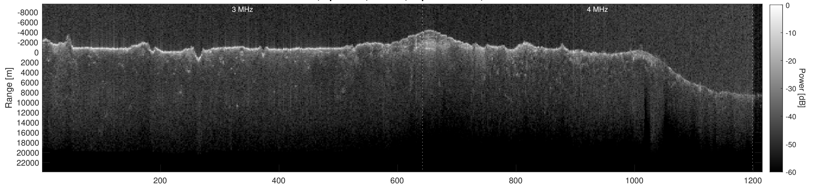
Orbit 2580, Depth-Corrected Cluttergram
