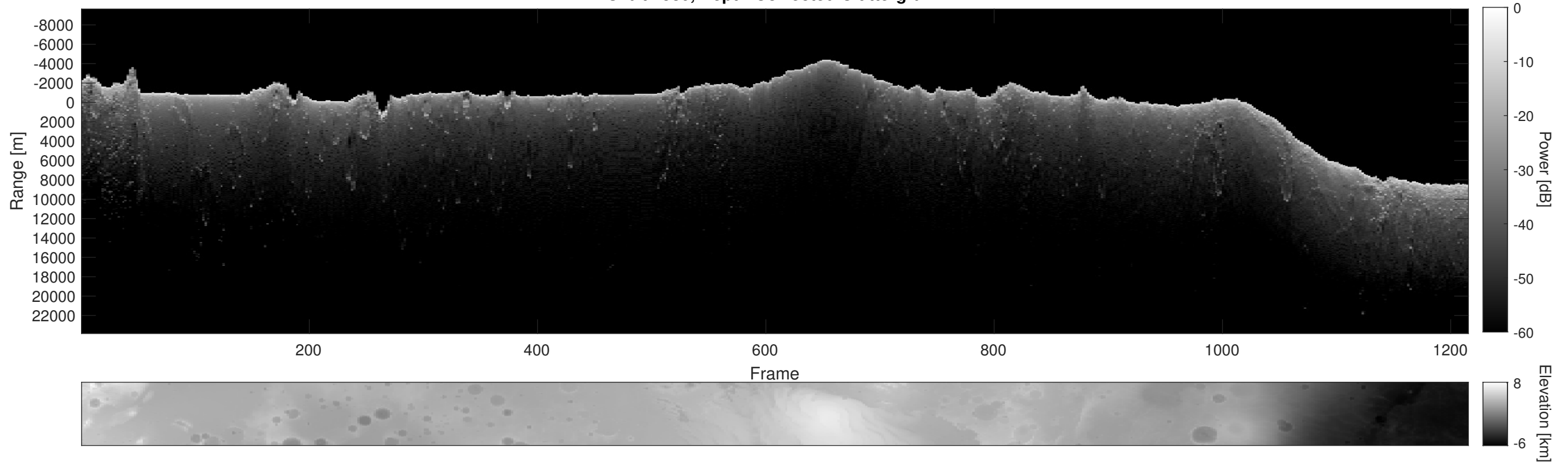
Orbit 2580, Depth-Corrected Cluttergram
