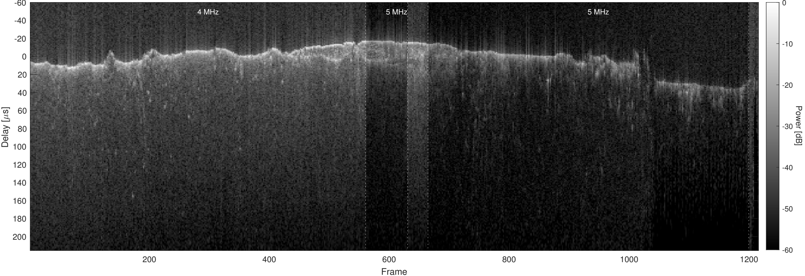
Orbit 2581, Optimized, No Window, Channel 2
