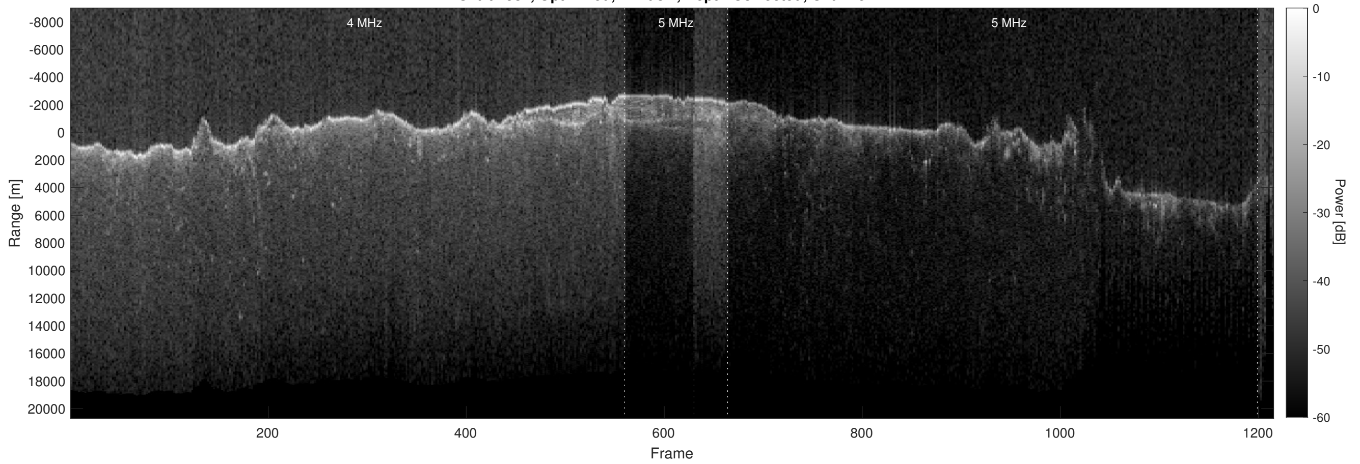
Orbit 2581, Optimized, Window, Depth-Corrected, Channel 2
