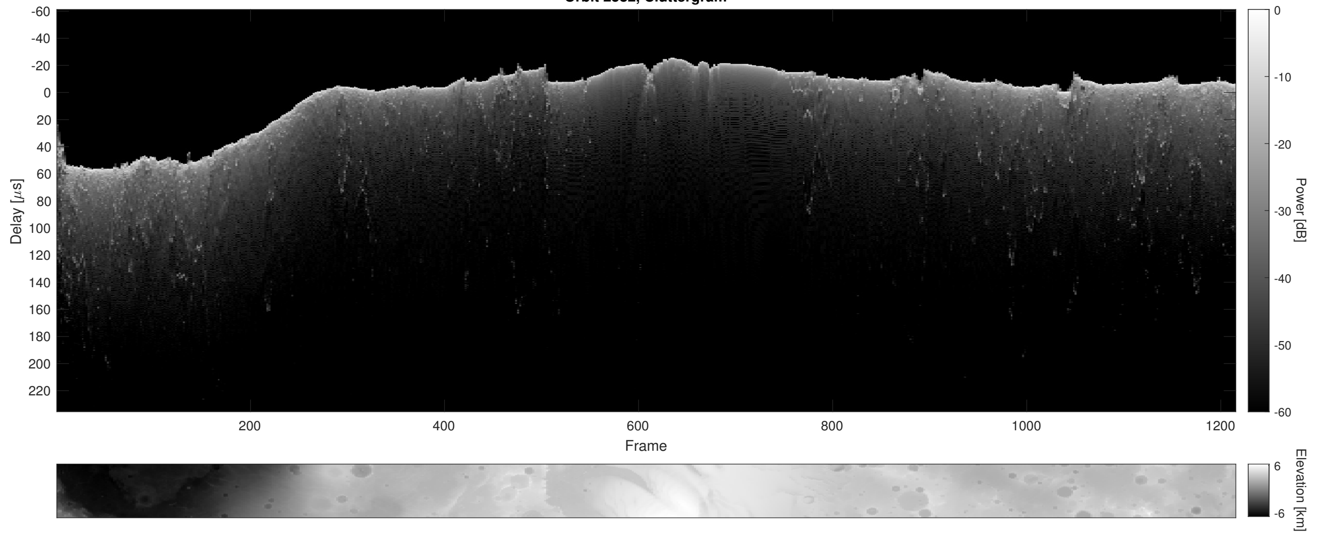
Orbit 2582, Cluttergram
