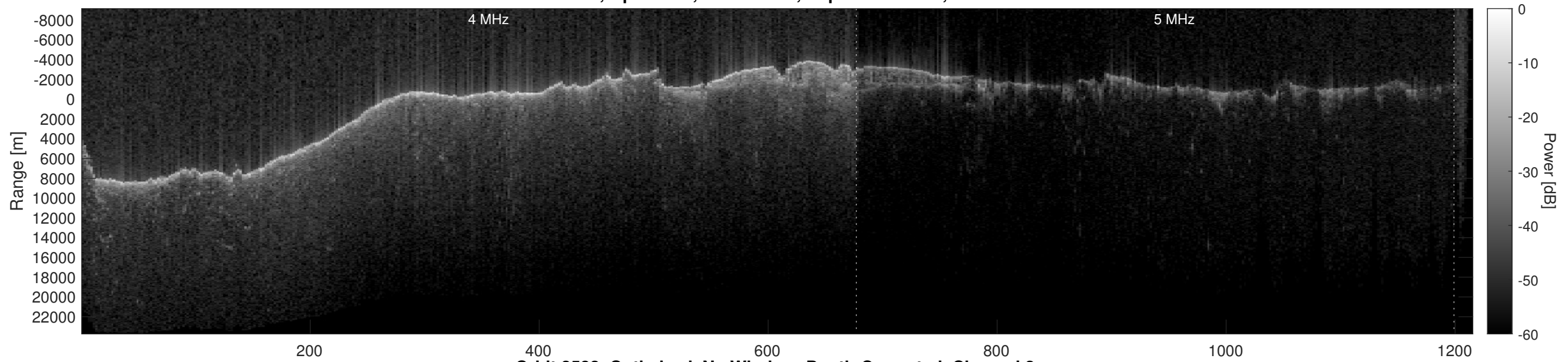
Orbit 2582, Optimized, No Window, Depth-Corrected, Channel 2
