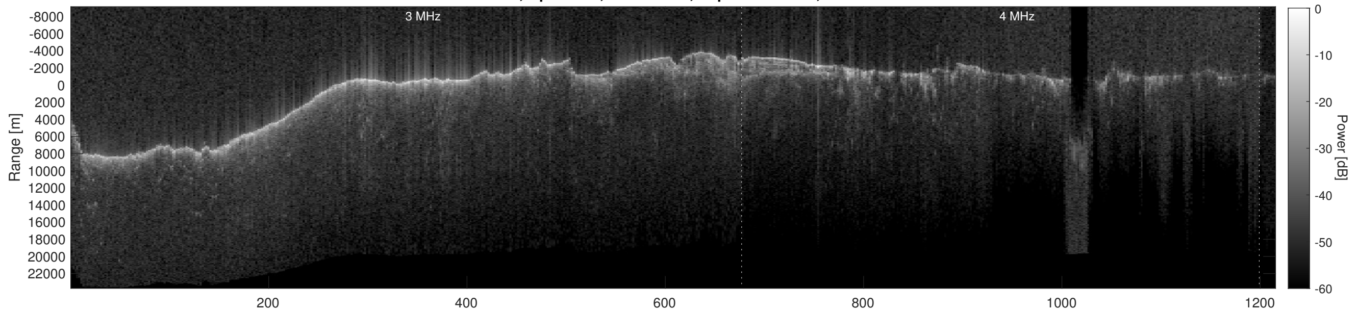
Orbit 2582, Depth-Corrected Cluttergram
