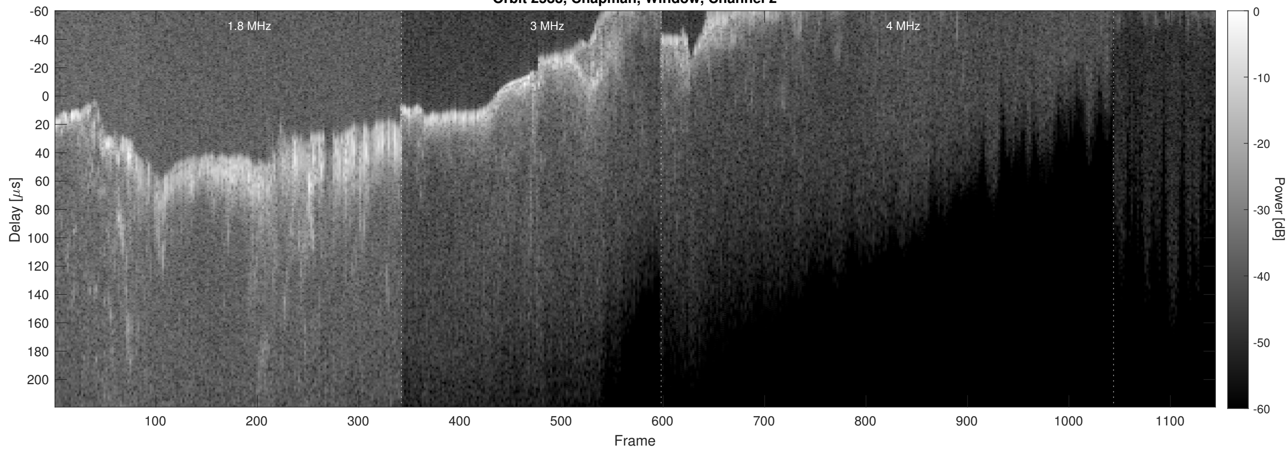
Orbit 2583, Chapman, Window, Channel 2
