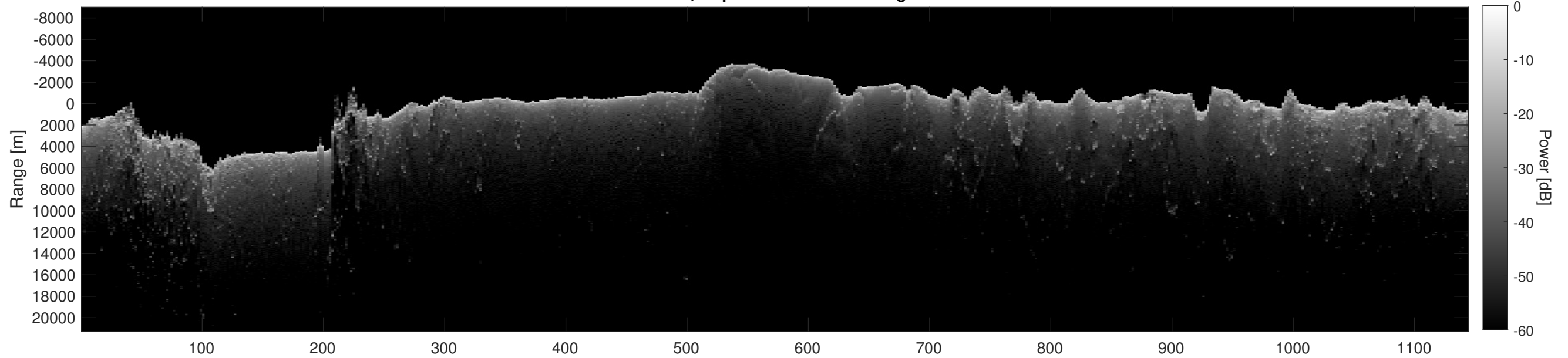
Orbit 2583, Depth-Corrected Cluttergram
