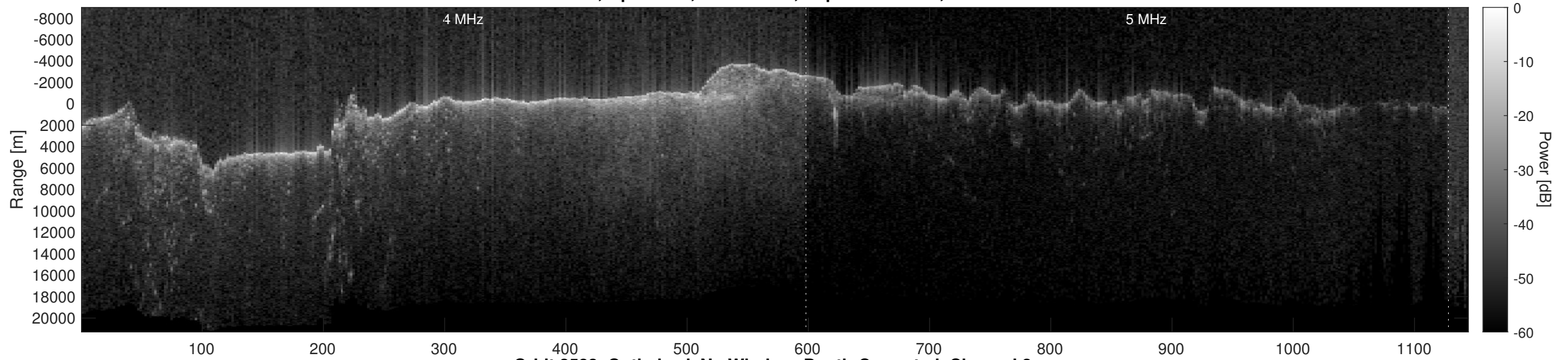
Orbit 2583, Optimized, No Window, Depth-Corrected, Channel 2
