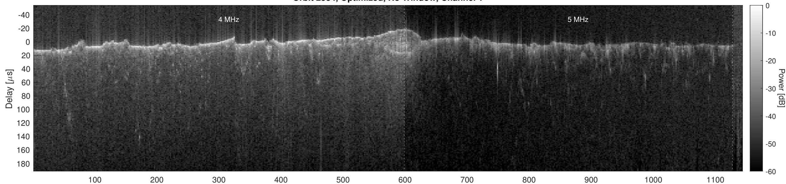
Orbit 2584, Optimized, No Window, Channel 2
