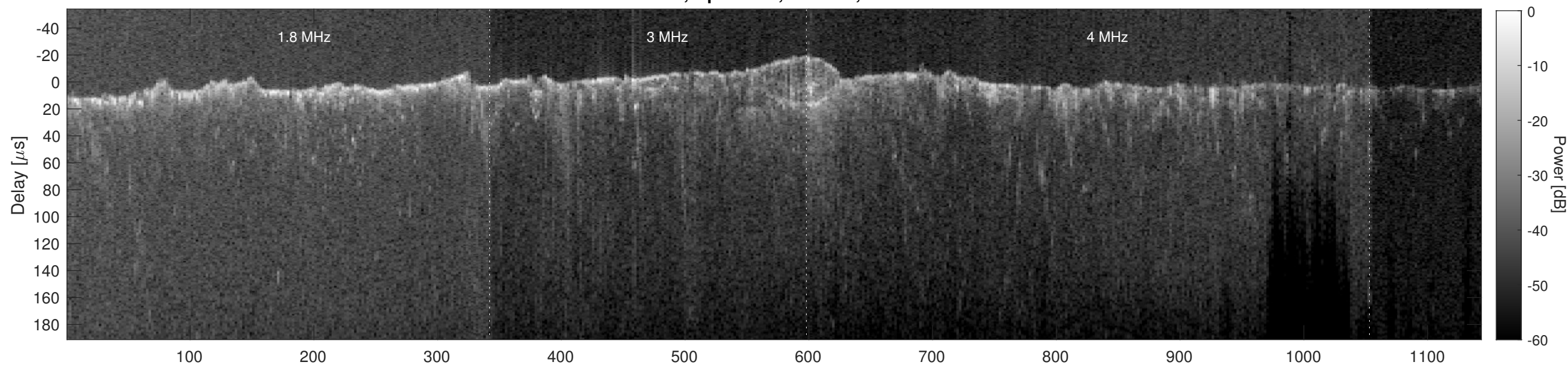
Orbit 2584, Cluttergram
