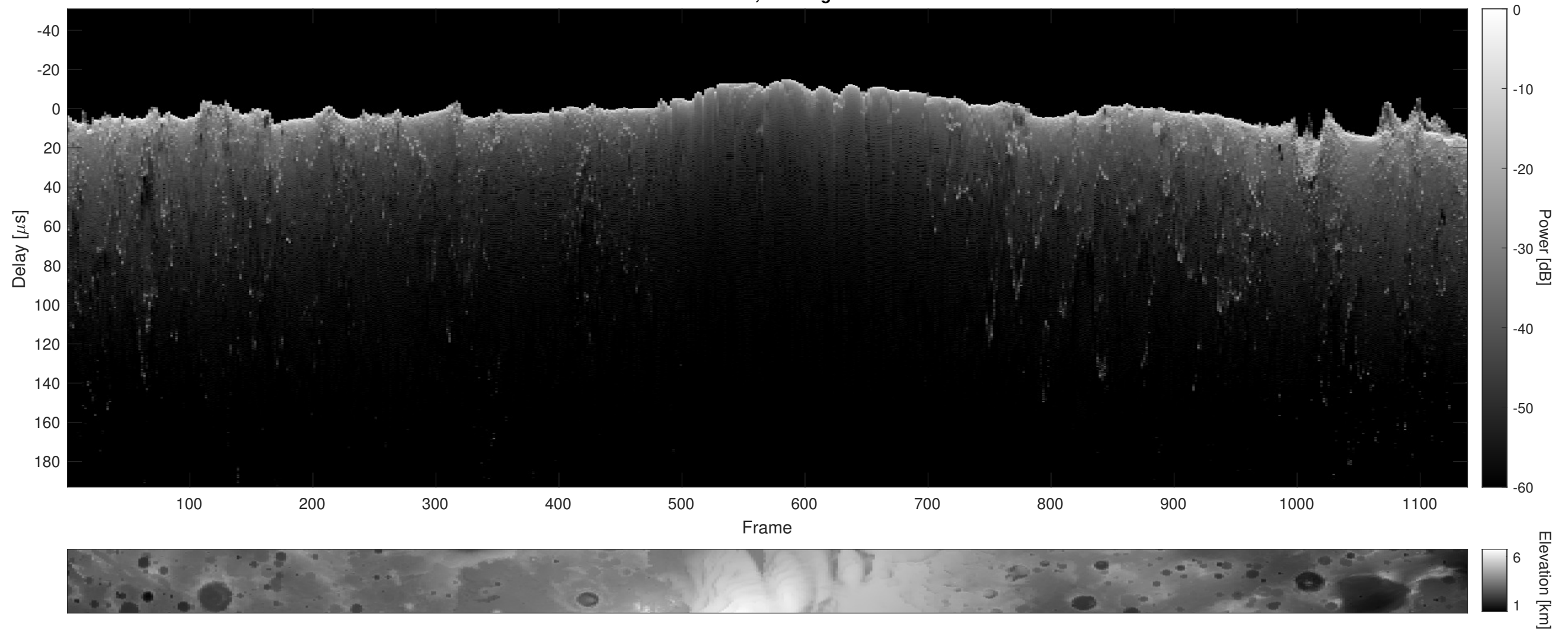
Orbit 2586, Cluttergram
