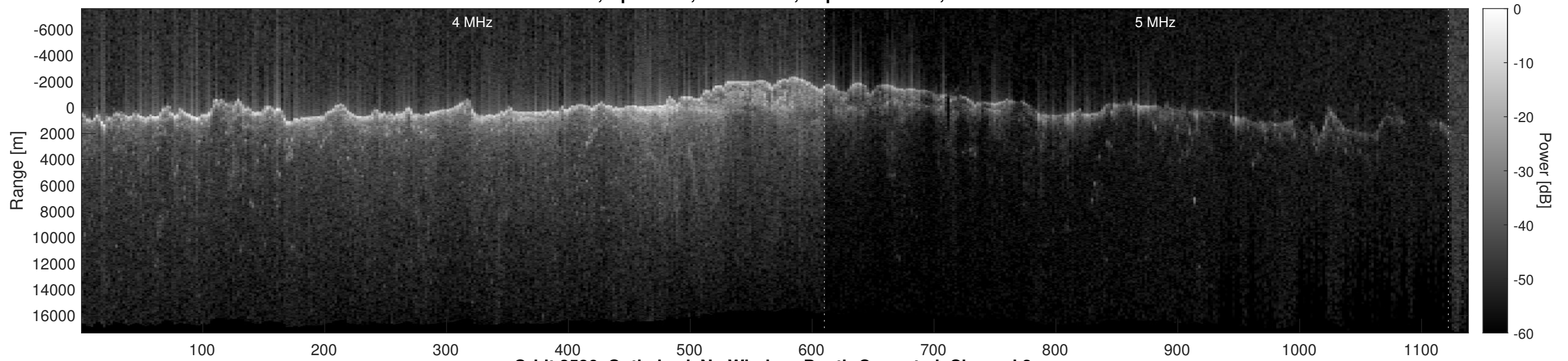
Orbit 2586, Optimized, No Window, Depth-Corrected, Channel 2
