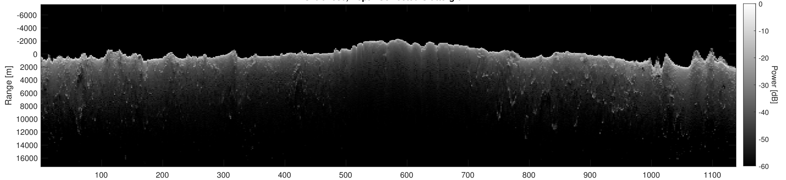
Orbit 2586, Depth-Corrected Cluttergram
