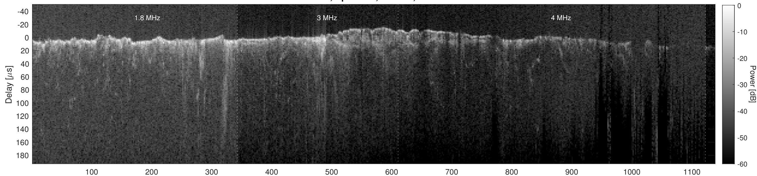
Orbit 2586, Cluttergram
