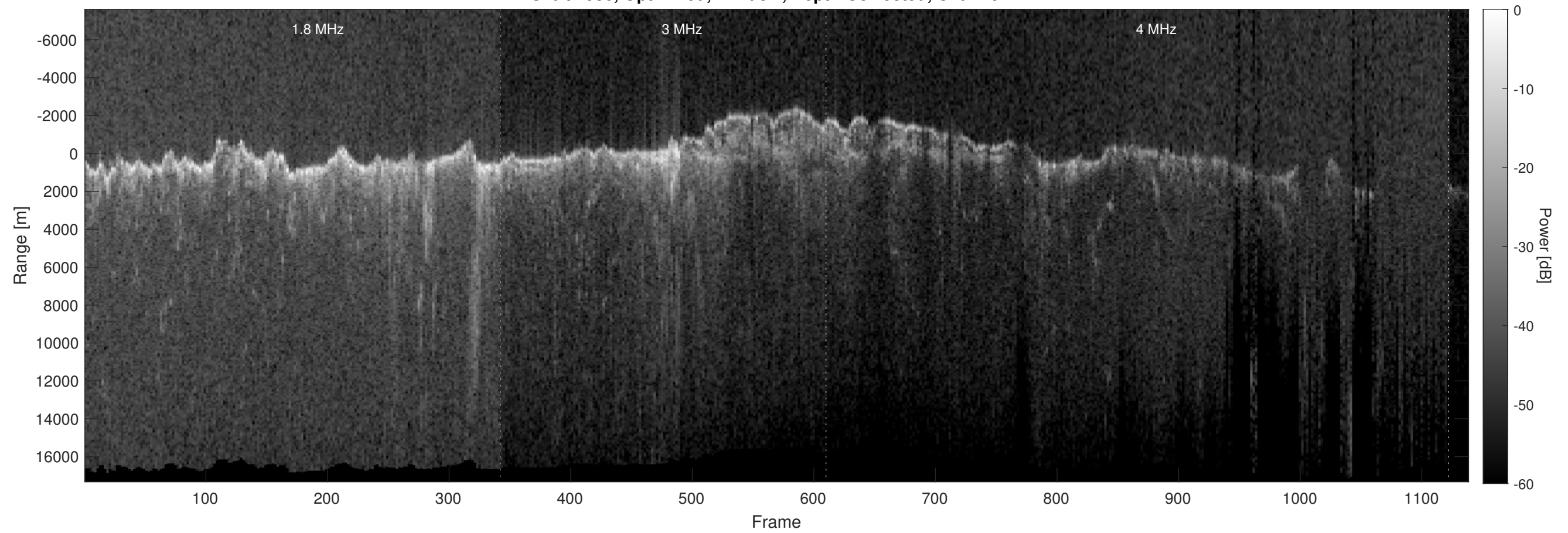
Orbit 2586, Optimized, Window, Depth-Corrected, Channel 2
