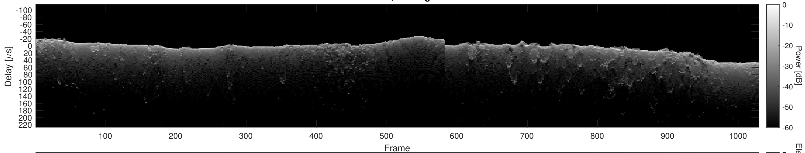
Orbit 2587, Cluttergram
