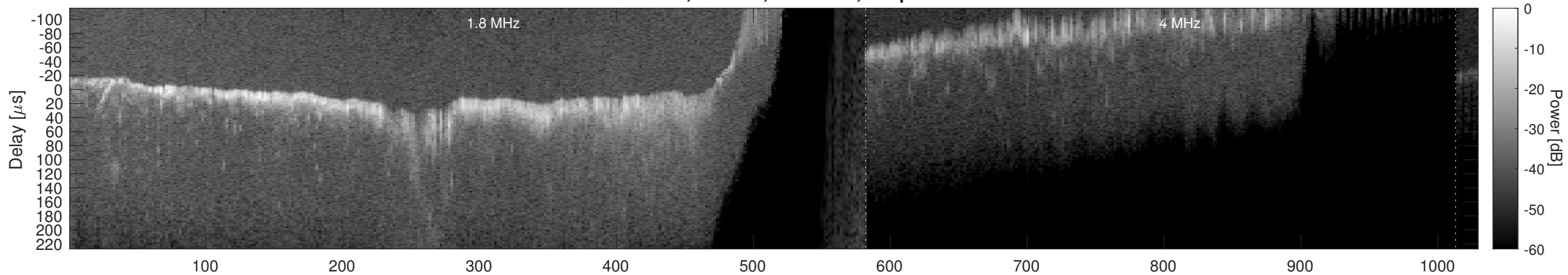
Orbit 2587, Window, Channel 2, Optimized
