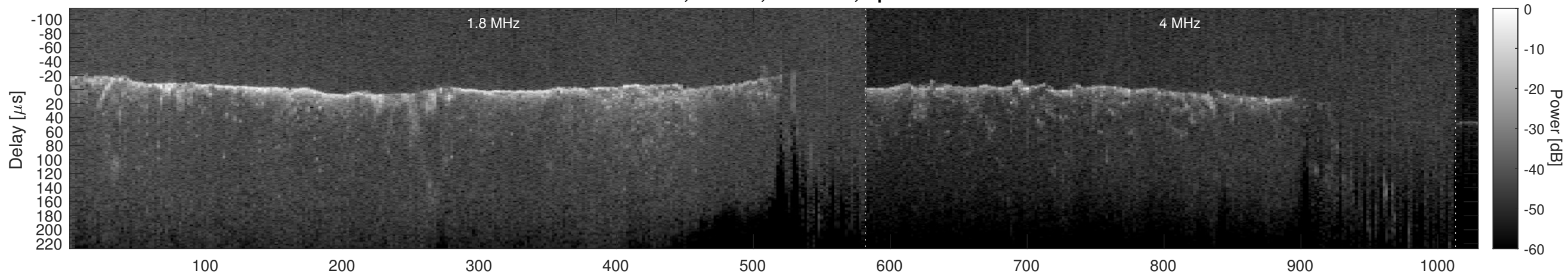
Orbit 2587, Cluttergram
