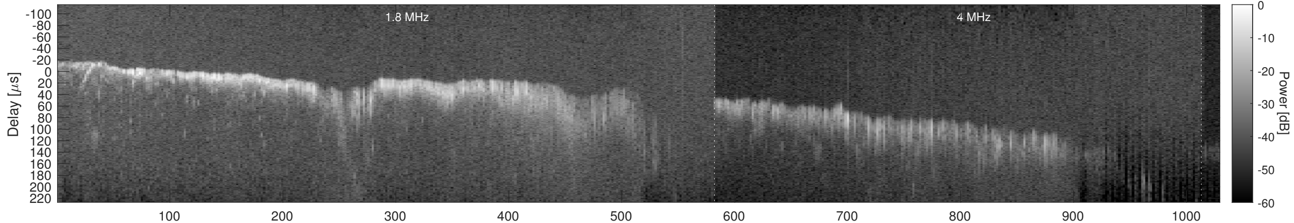
Orbit 2587, Window, Channel 2, Chapman
