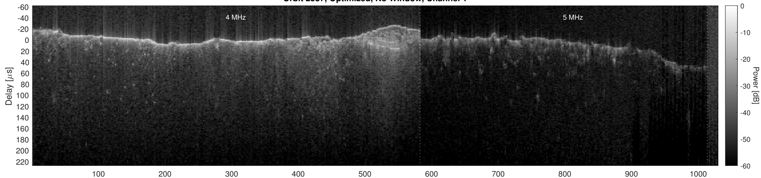
Orbit 2587, Optimized, No Window, Channel 2
