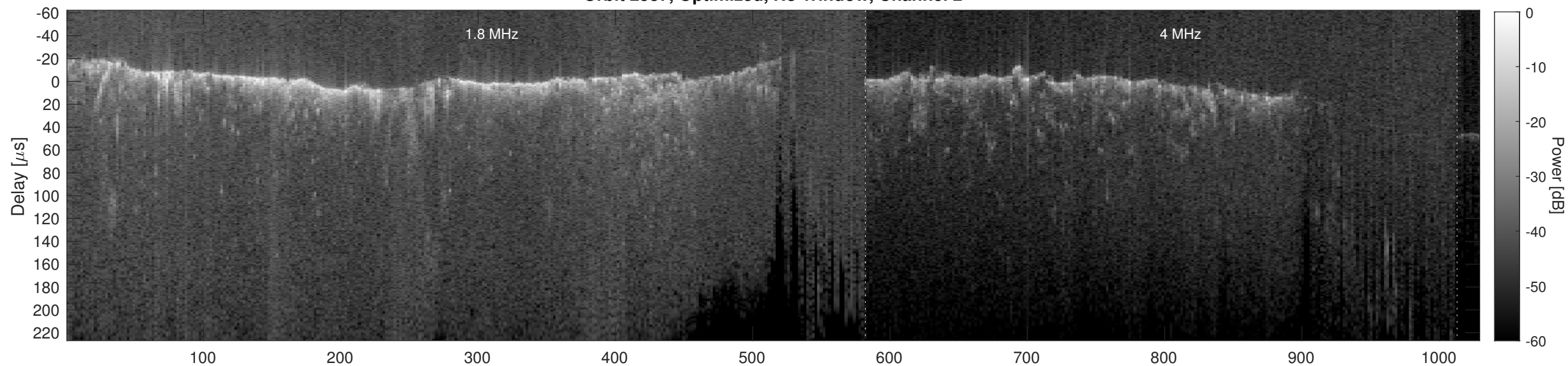
Orbit 2587, Cluttergram
