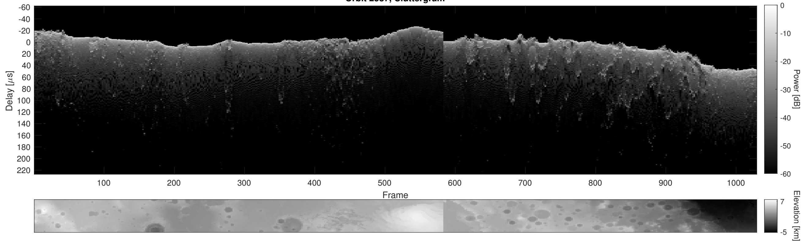
Orbit 2587, Cluttergram
