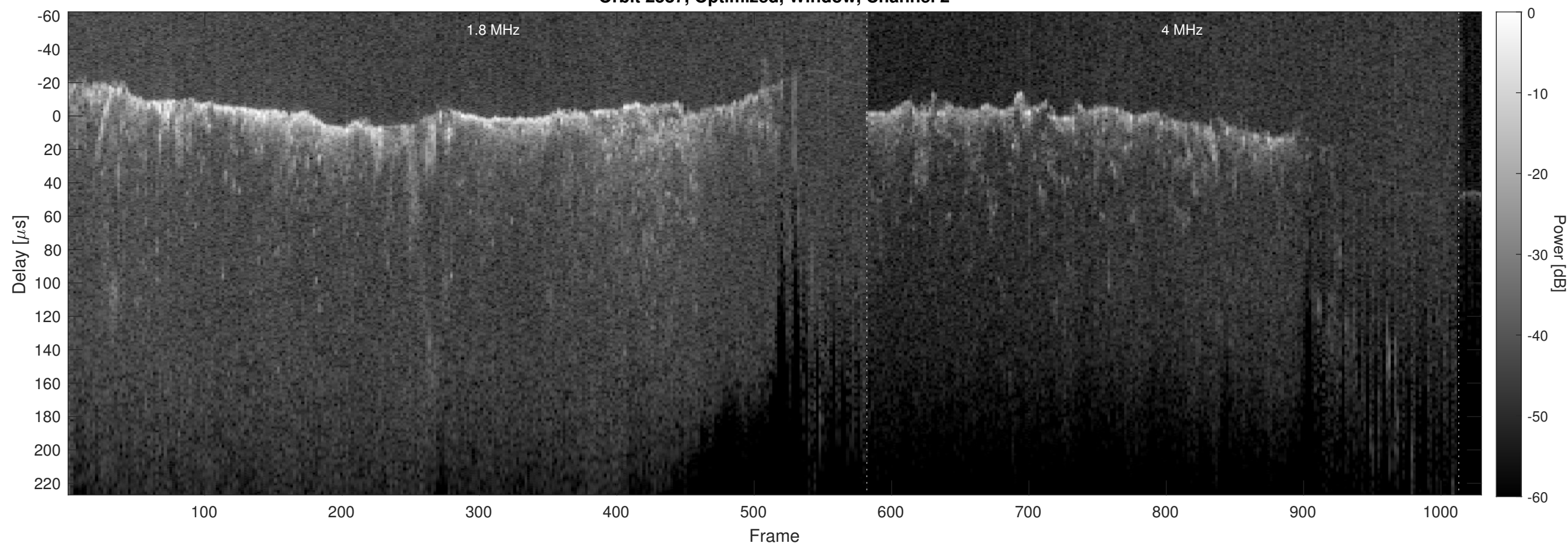
Orbit 2587, Optimized, Window, Channel 2
