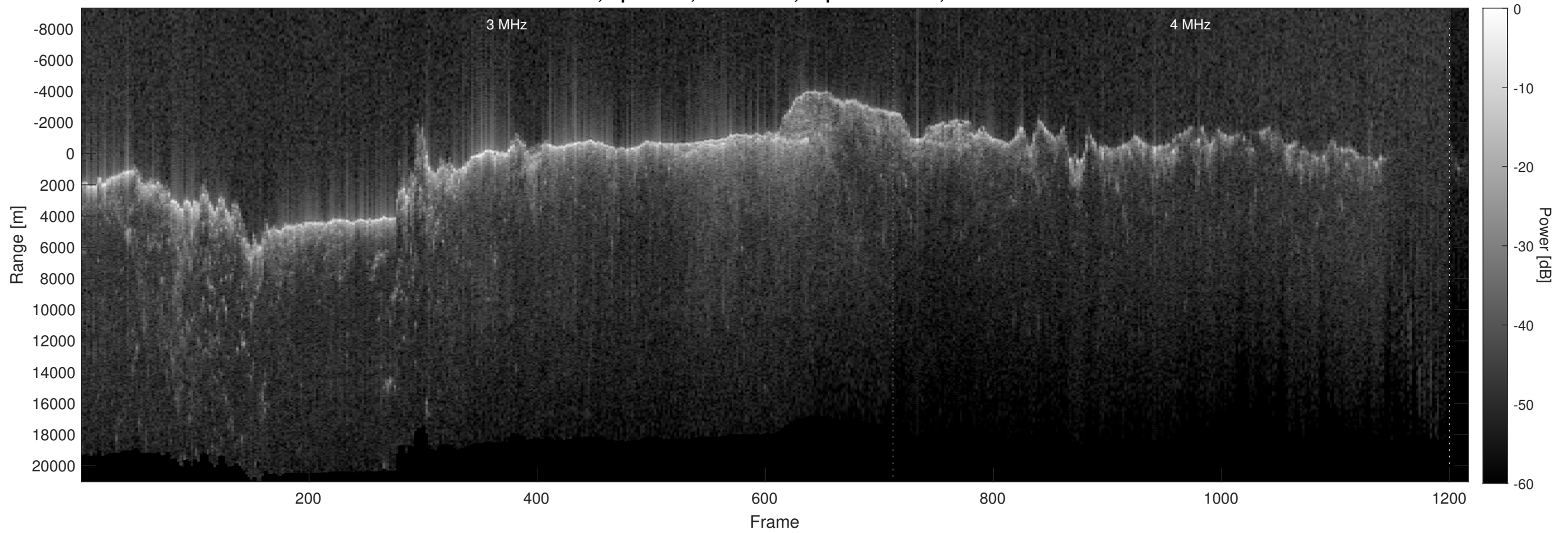
Orbit 2594, Optimized, No Window, Depth-Corrected, Channel 2
