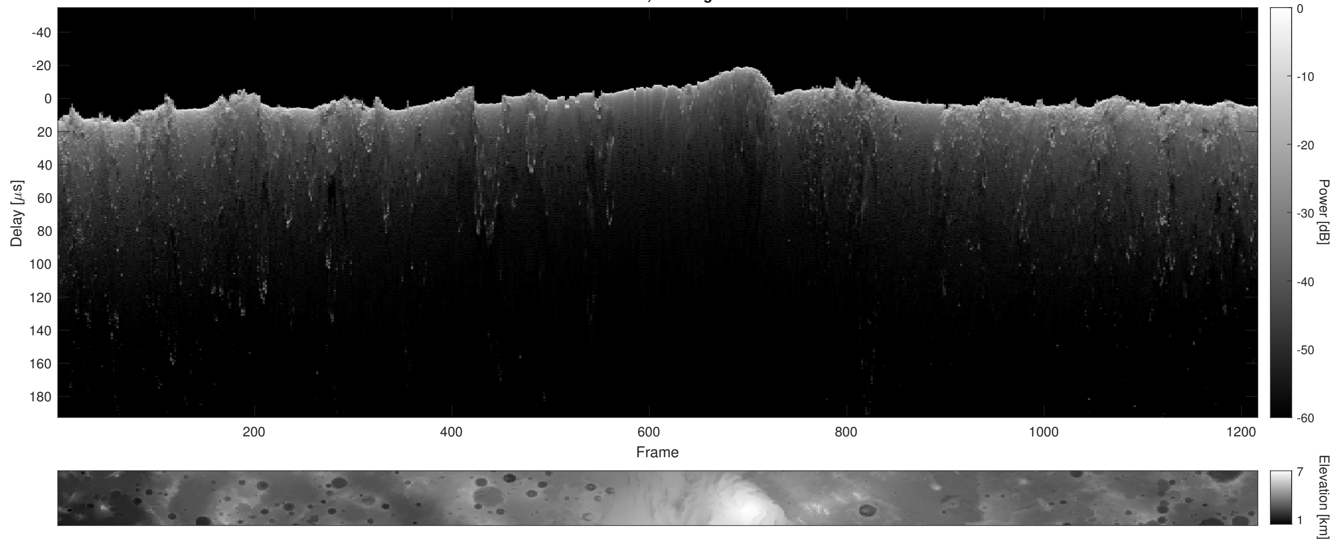
Orbit 2595, Cluttergram
