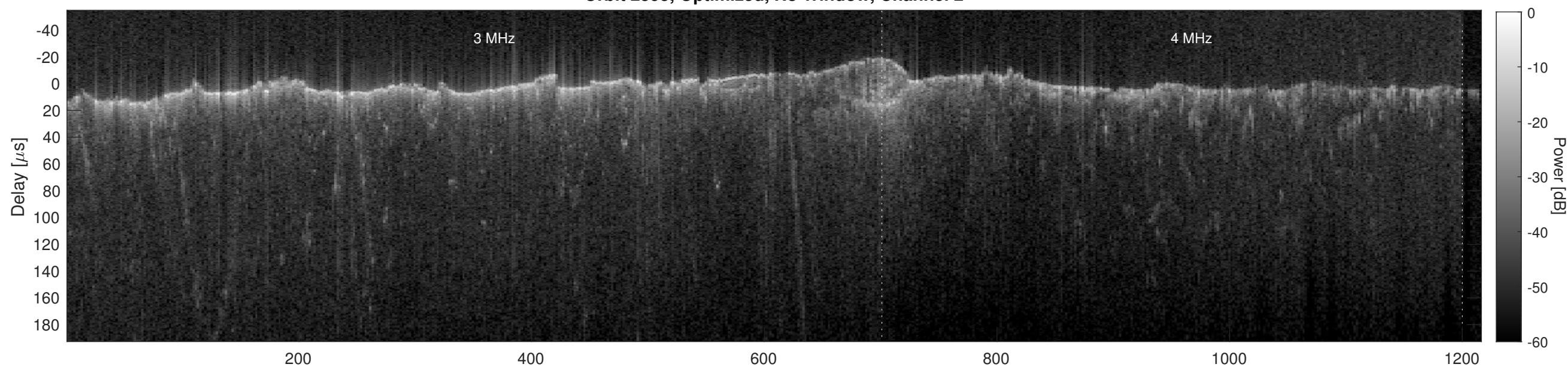
Orbit 2595, Cluttergram
