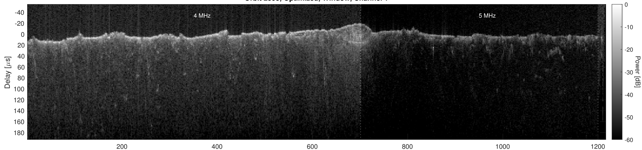
Orbit 2595, Optimized, Window, Channel 2
