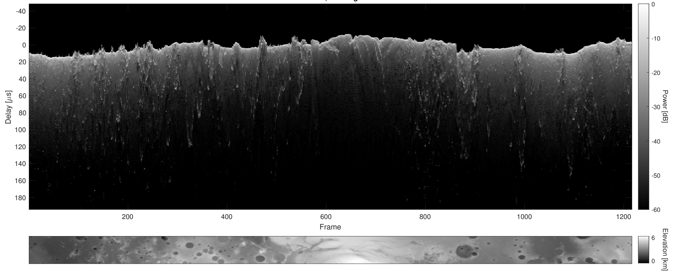
Orbit 2596, Cluttergram
