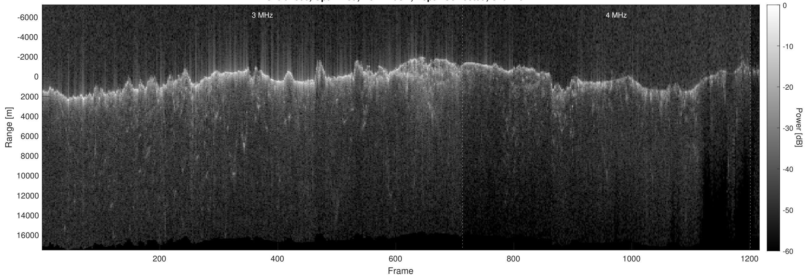
Orbit 2596, Optimized, No Window, Depth-Corrected, Channel 2
