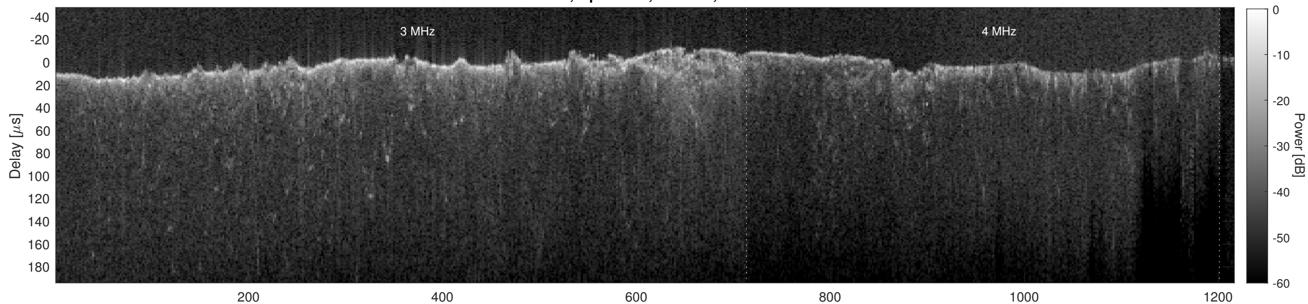
Orbit 2596, Cluttergram
