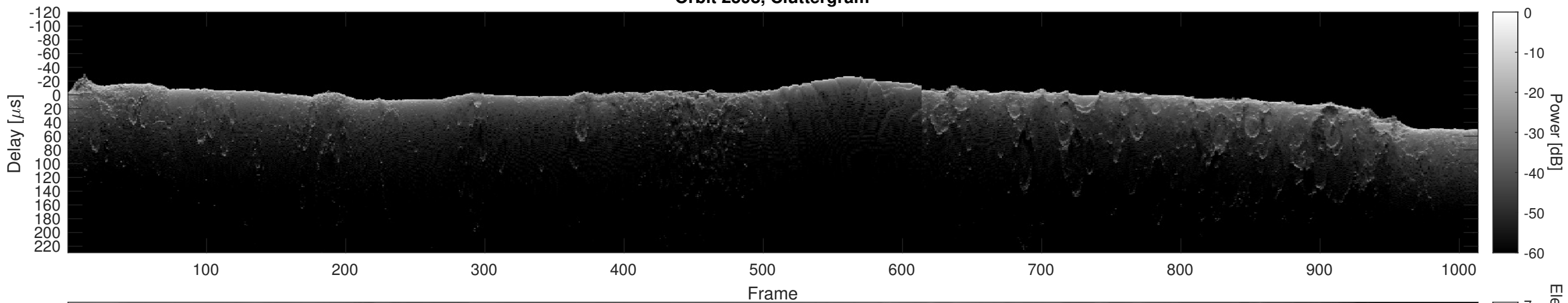
Orbit 2598, Cluttergram
