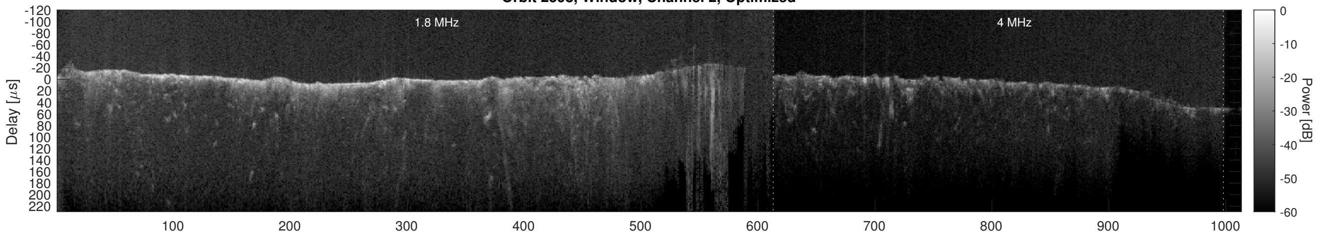
Orbit 2598, Cluttergram
