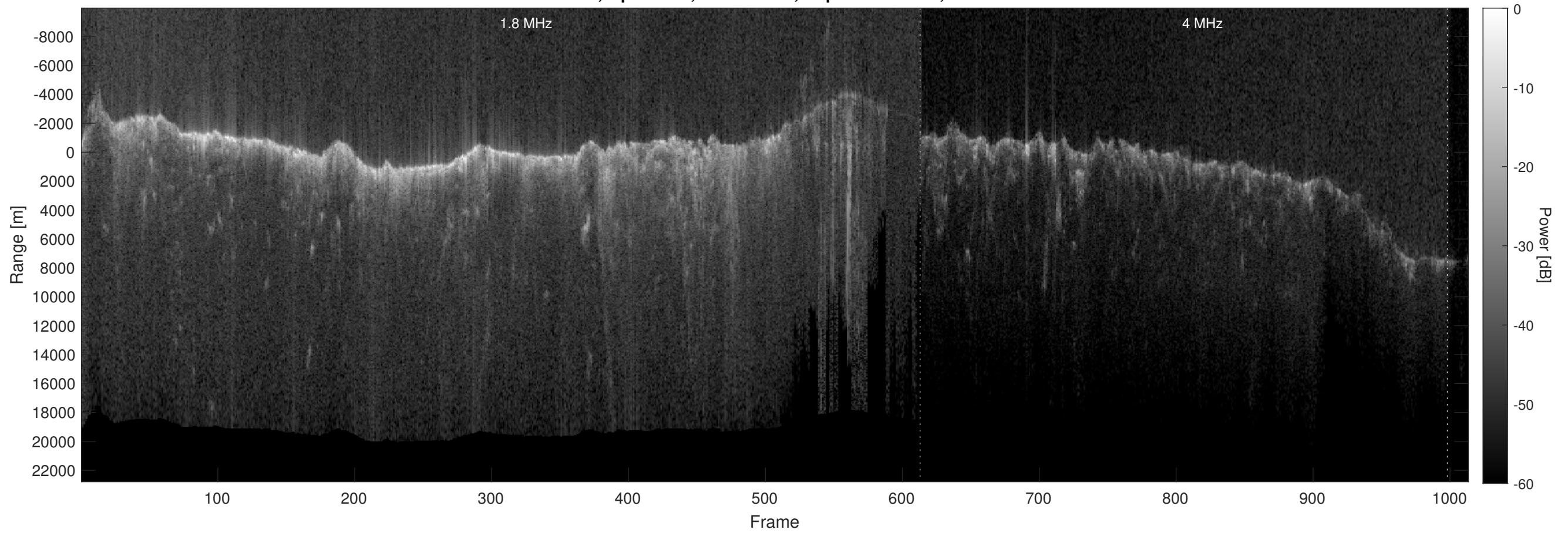
Orbit 2598, Optimized, No Window, Depth-Corrected, Channel 2
