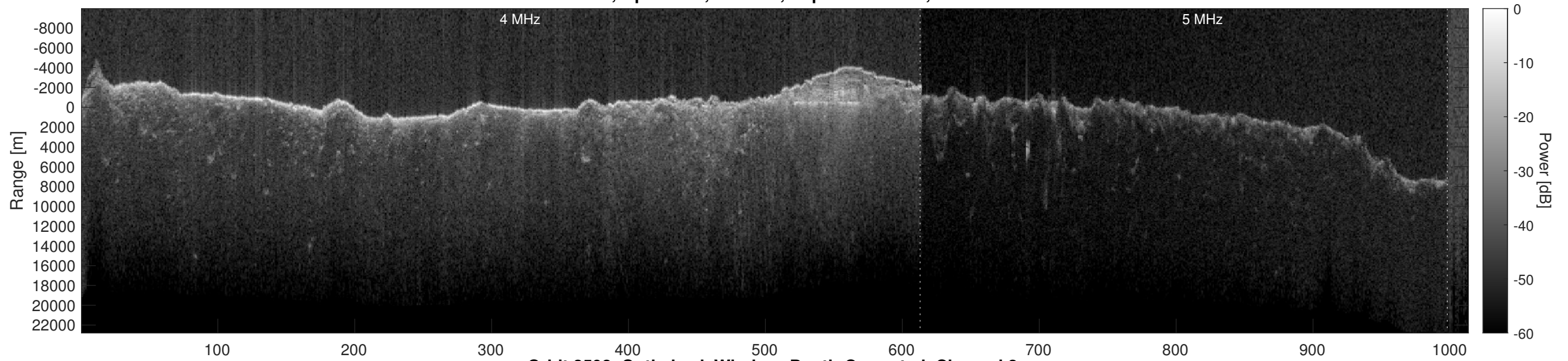
Orbit 2598, Optimized, Window, Depth-Corrected, Channel 2
