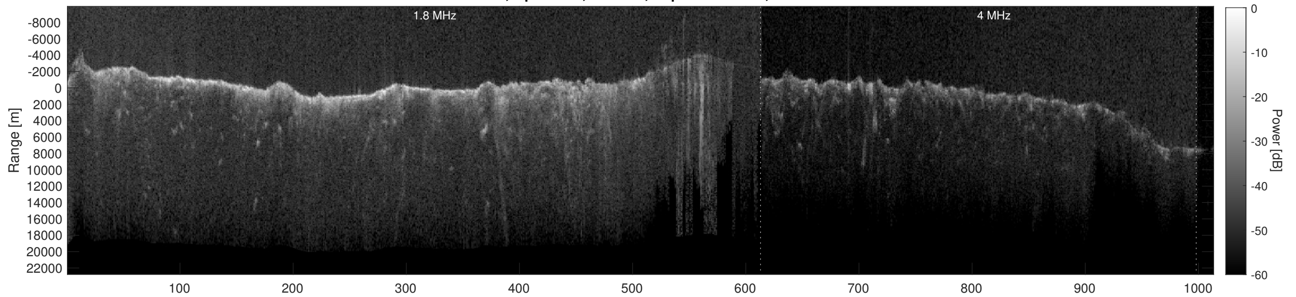
Orbit 2598, Depth-Corrected Cluttergram
