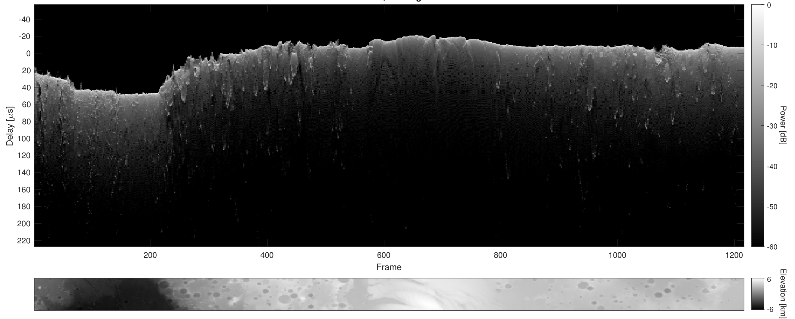
Orbit 2600, Cluttergram
