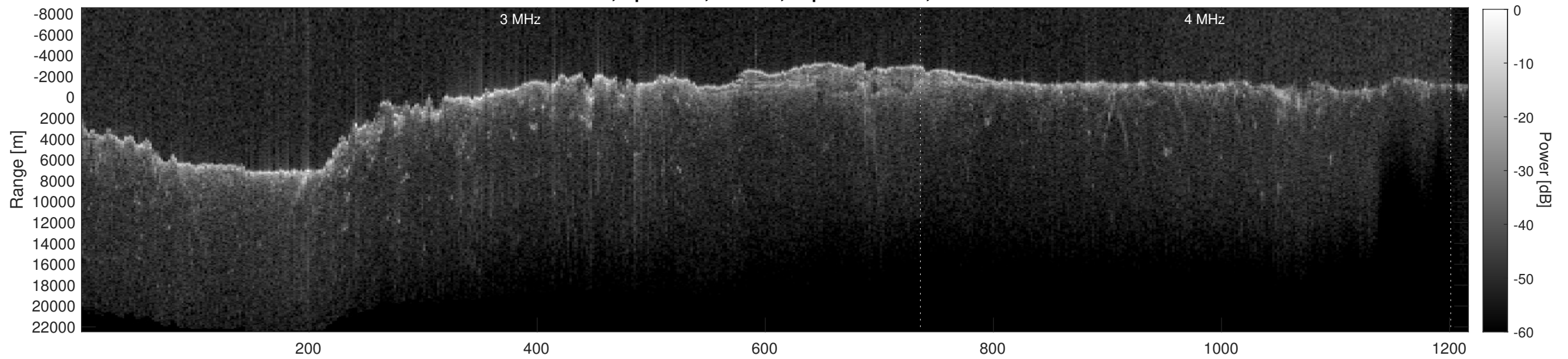
Orbit 2600, Depth-Corrected Cluttergram
