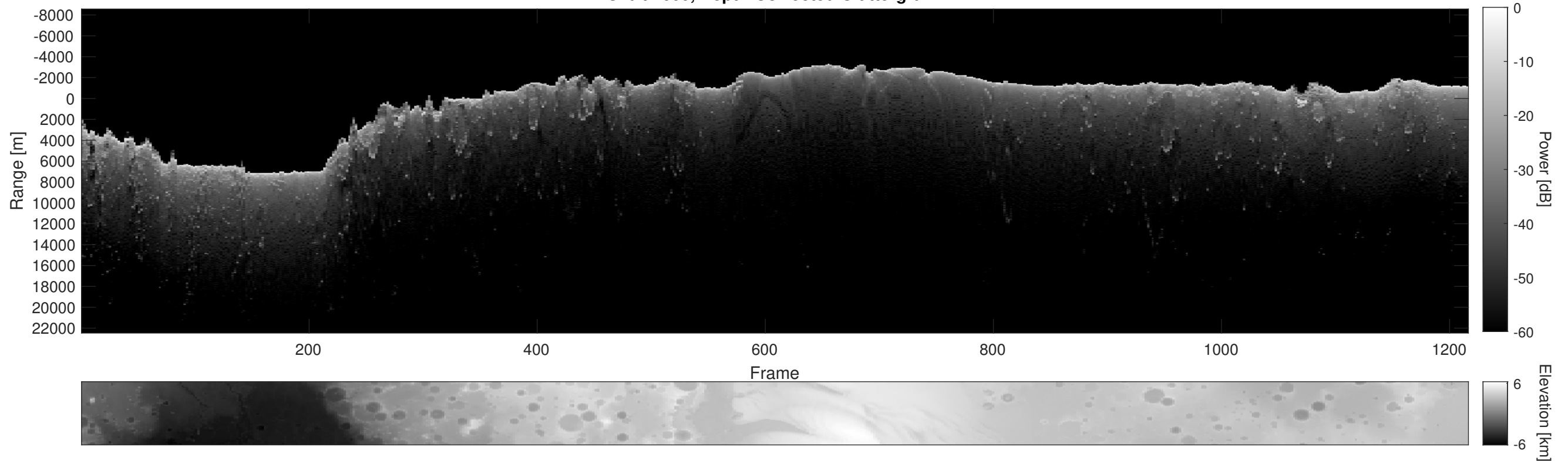
Orbit 2600, Depth-Corrected Cluttergram
