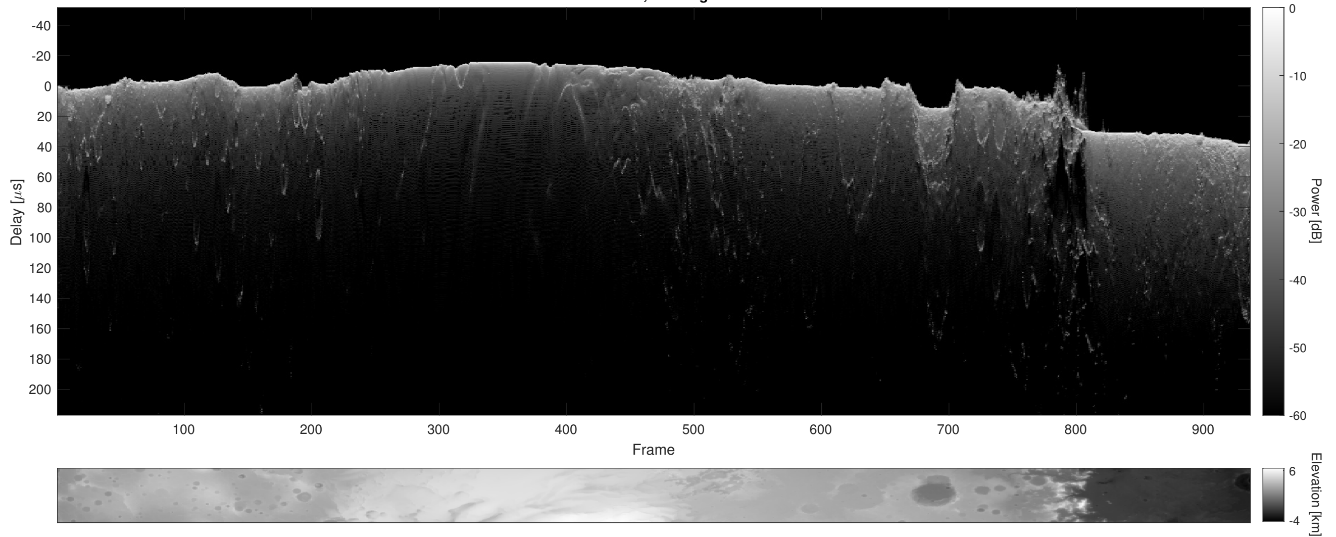
Orbit 2603, Cluttergram
